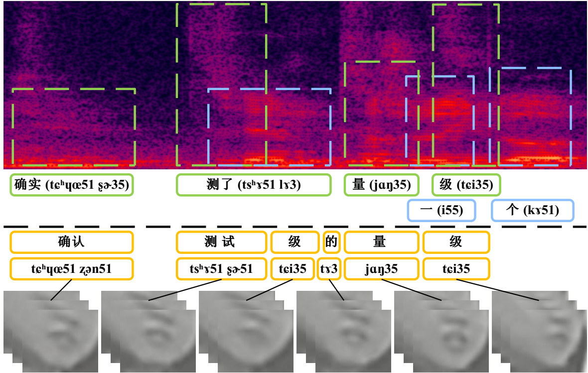
(c) Far-field Speech, Lip Frames and Aligned Recognitions Result of Target Speaker
